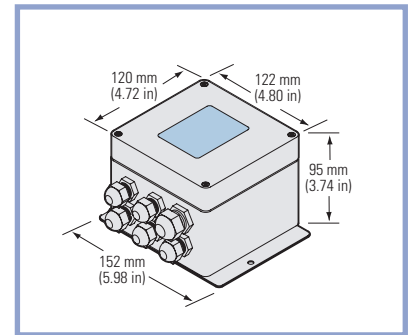
Power Pack
