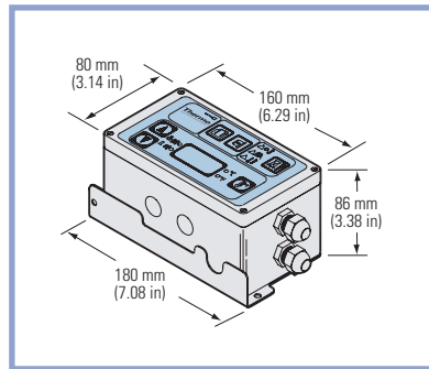
Control Module
